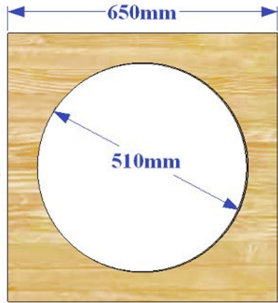
Inner baffle
